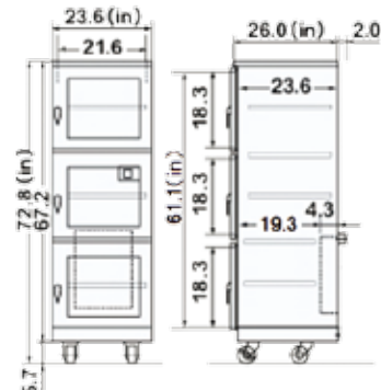
DXU-501A 22 cf (3-door type)
